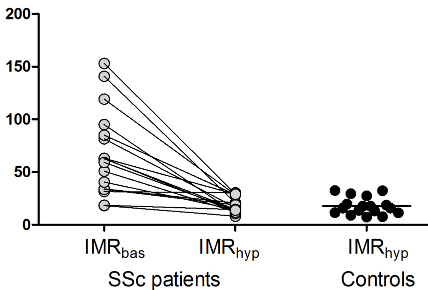
Figure 4: In systemic sclerosis (SSc) patients the myocardial resistance at maximal vasodilatation ( IMR_{hyp} ) was not significantly different from controls ( p=0.99 ). The difference of the magnitude of the response to vasodilatation (i.e. the coronary flow reserve) is dominated by the differences in the resting resistance ( IMR_{bas} ) i.e. in the vascular tone.
