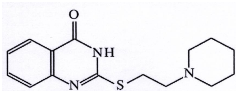
Figure 1. Chemical structure of L-2286 (2-[(2-piperidine-1-yl)thio]quinazolin-4(3H)-one).
